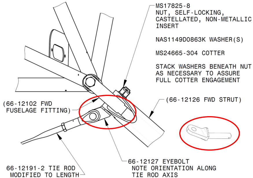
VIEW FROM FRONT OF AIRCRAFT SHOWING FWD STRUT AND FITTING INSTALLATION FUSELAGE SKIN HIDDEN FOR CLARITY
